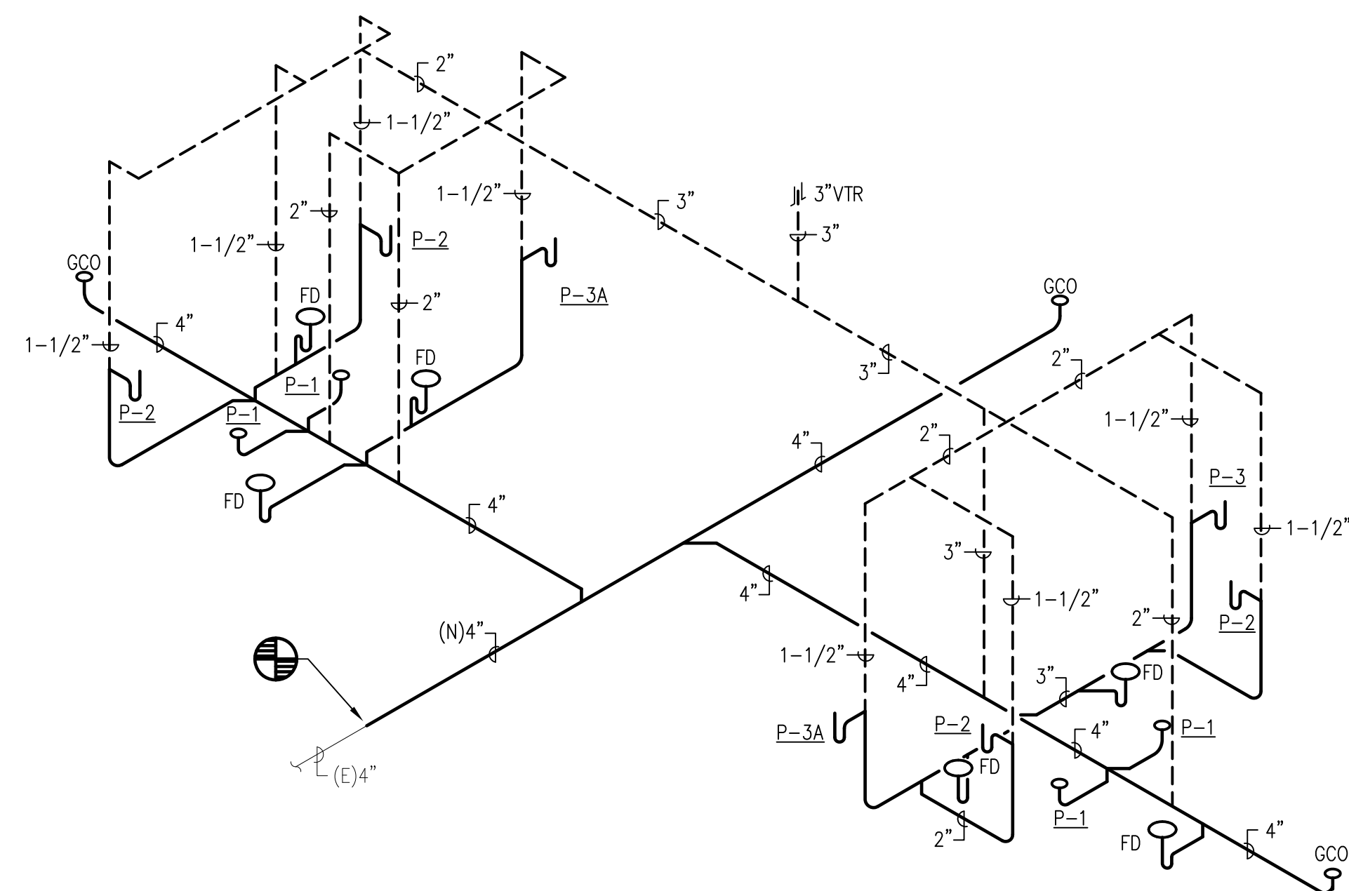
SANITARY SEWER RISER DIAGRAM
